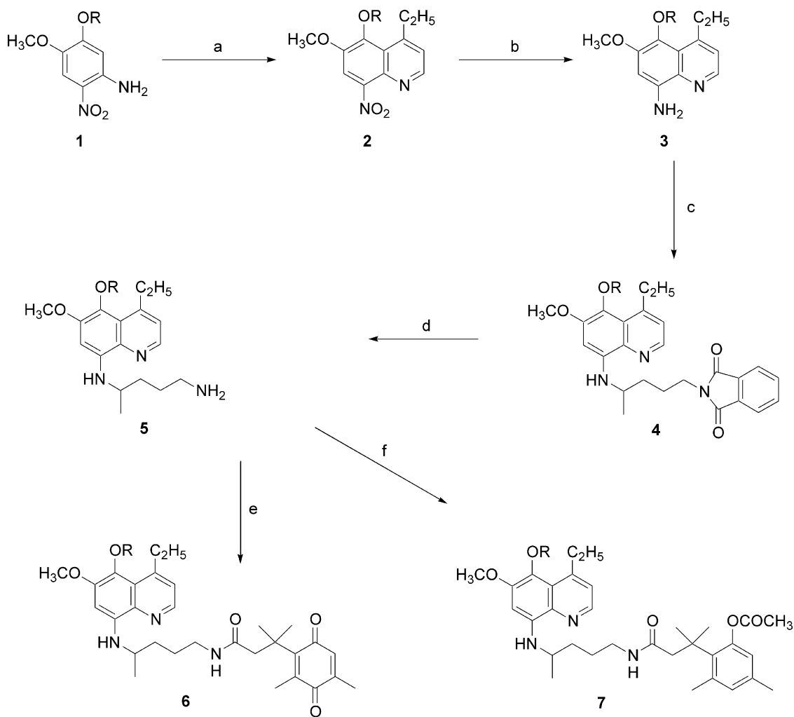
Scheme 1. (a) 1-Chloro-3-pentanone, 85% o -H 3 PO 4 , As 2 O 5 , 80 °C, 3 h; (b) Raney nickel, EtOH, H 2 , 45 psi, 45 min; (c) 2-(4-bromopentyl)-1,3-isoindolinedione, Et 3 N, 120 °C, 24 h; (d) NH 2 NH 2 ·H 2 O, EtOH, reflux, 8 h; (e) 3-(2,4-dimethyl-3,6-dioxo-1,4-cyclohexadienyl)-3-methylbutanoic acid ( 8 ), DCC, DMAP, DCM, 4 h; (f) 3-(2,4-dimethyl-6-methylcarbonyloxyphenyl)-3-methylbutanoic acid ( 9 ), DCC, DMAP, DCM, 4 h.
